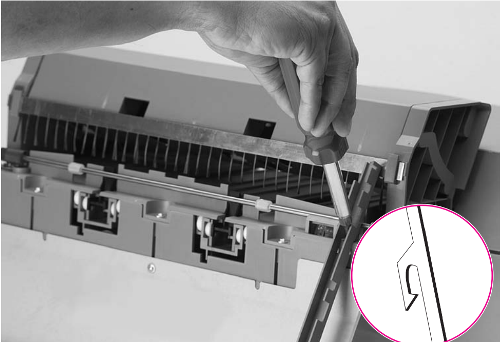
Figure 6-182 Back Plate (1 of 2)
